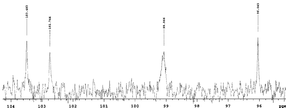
Figure 3. Expanded ^{13}\text{C} anomeric region of glycopolymer 15B .
