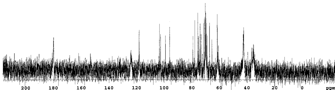
Figure 2. ^{13}\text{C} NMR spectrum of glycopolymer 15B on \text{D}_2\text{O} at room temperature.
